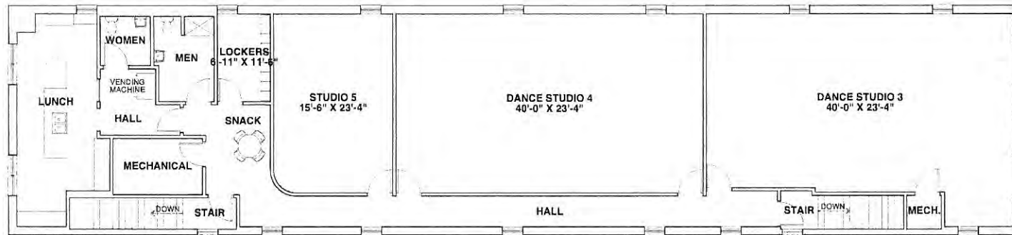
PRELIMINARY SECOND FLOOR PLAN
